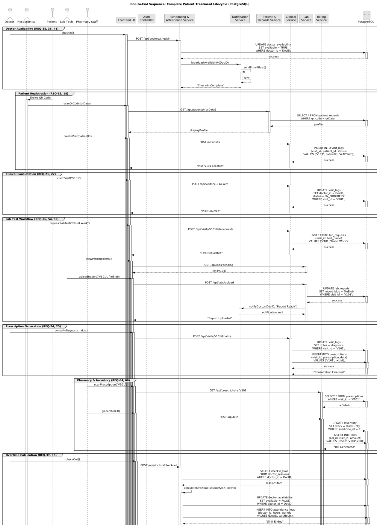
Fig. 13. Sequence diagram.
