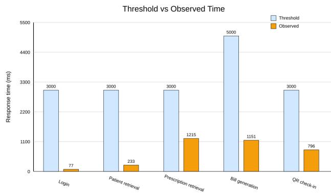
Fig. 4. Average measured backend response time by module from the current validation dataset.
