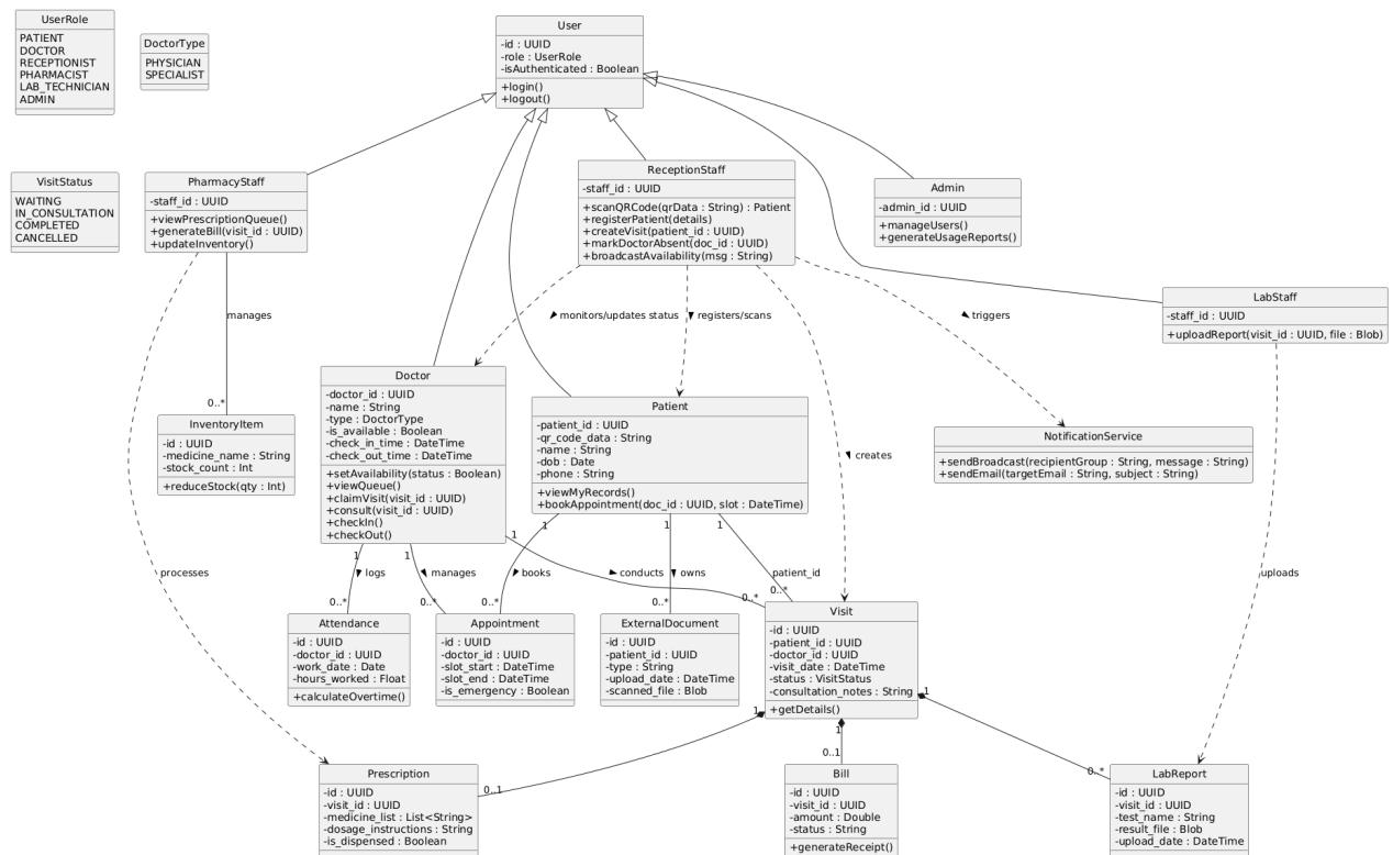
Fig. 9. Class diagram.
